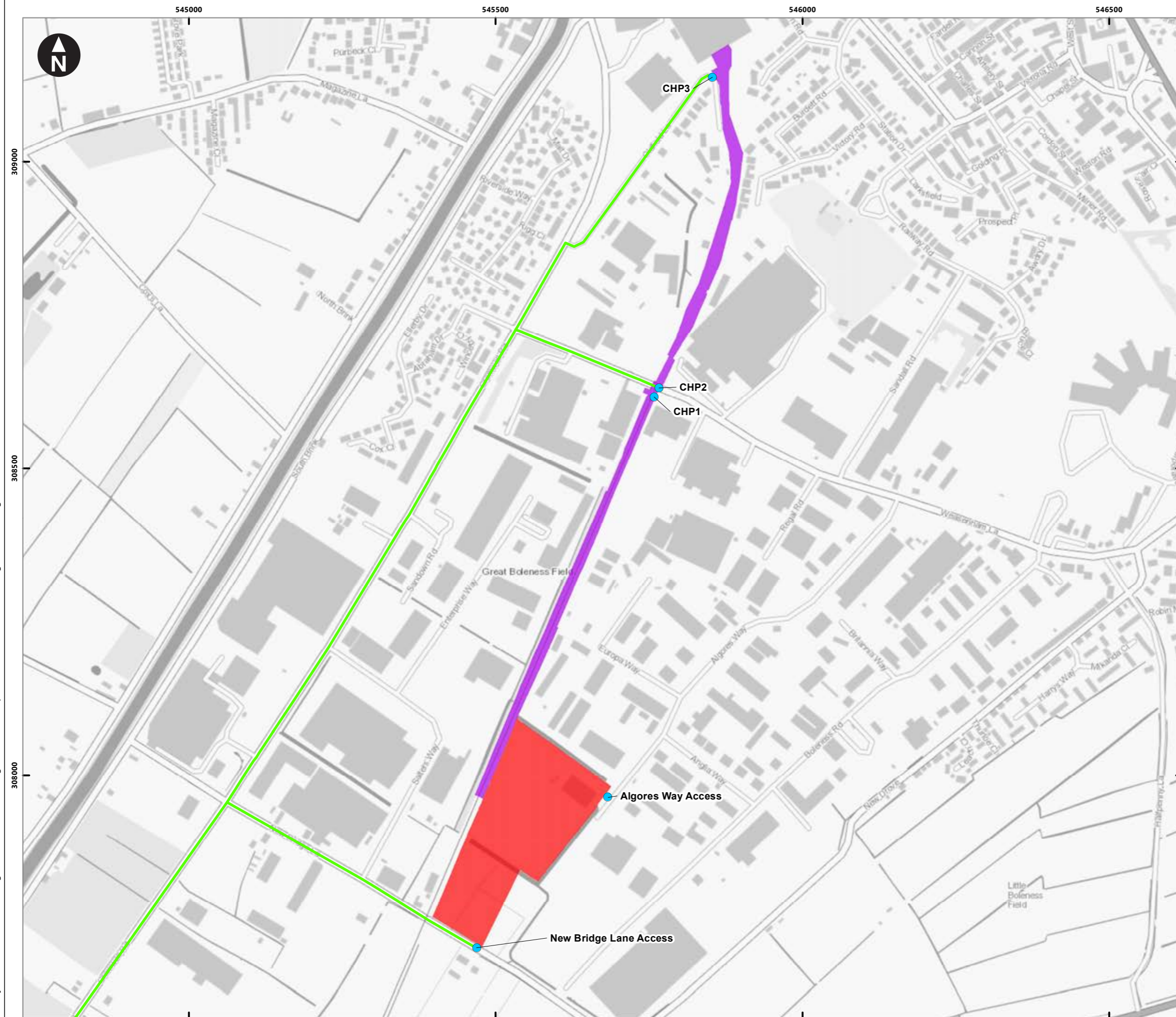
Figure 4.2 CHP Connection Access Strategy
