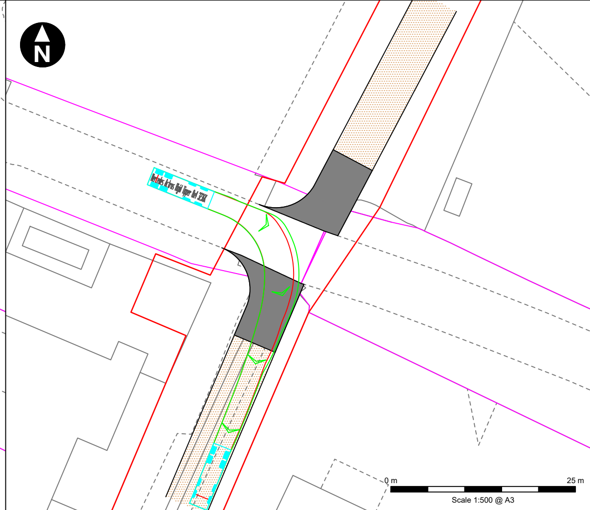
Figure 10.3ii Proposed Construction Access Weasenham Lane SPA
